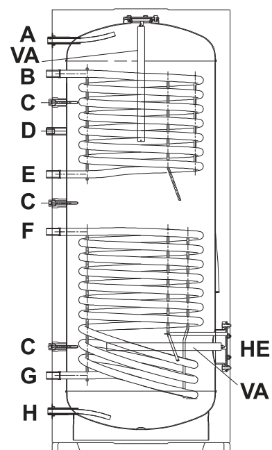
ECOUNIT 200/300 L-2C
