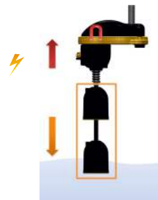
The water reaches the minimum level and the weight of the floating body disengages the magnet
