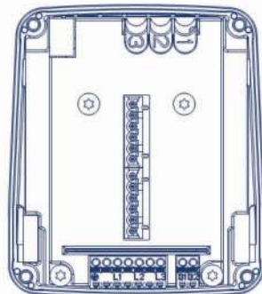
Fig 5: Electronics without speed selector
