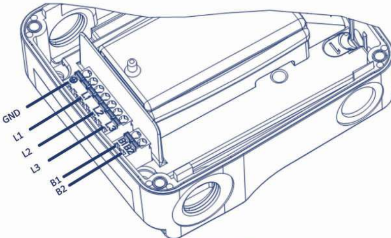
Figure 3: Electrical scheme
