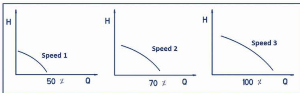
Fig 9: Characteristics of the pump at different speeds
