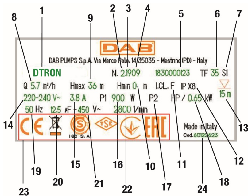
Image 4 Plaque
