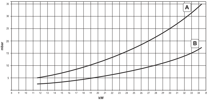
Pressure - power diagrams DIVatech D C32
