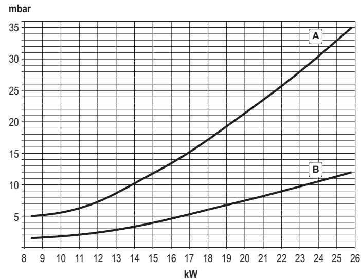
Circulating pump head / pressure losses DIVatech D C24
