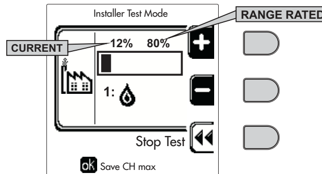
fig. 76 - Test mode (example heating power = 80%)
