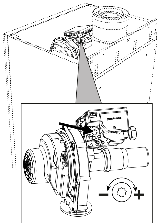
fig. 74- Minimum adjustment, models W 60 and W 80
