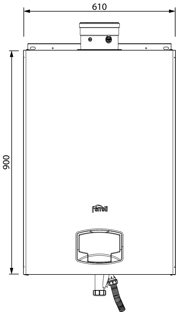
fig. 79- Front view
