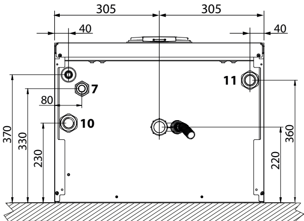
fig. 82- Top view
