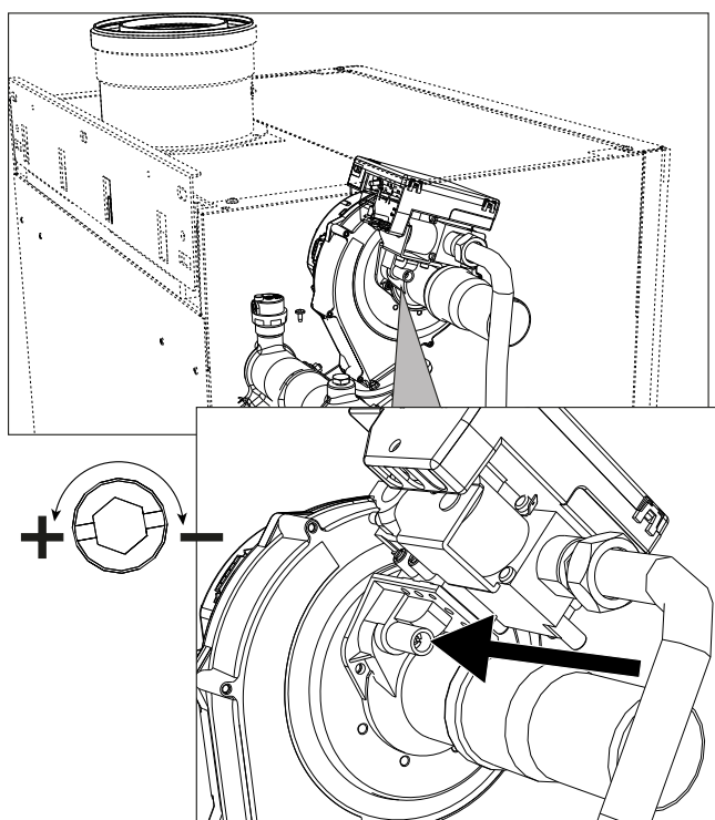
fig. 73- Maximum adjustment, models W 60 and W 80
