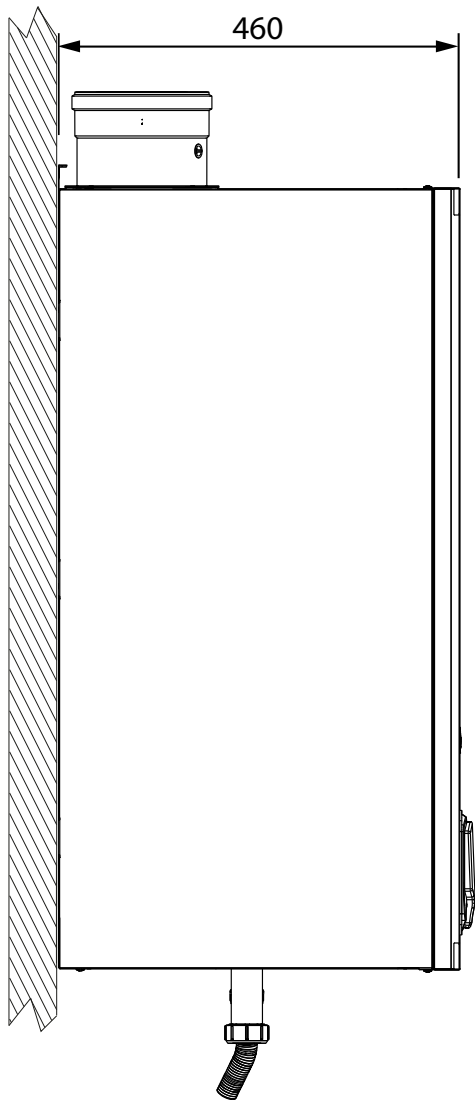
fig. 80- Side view
