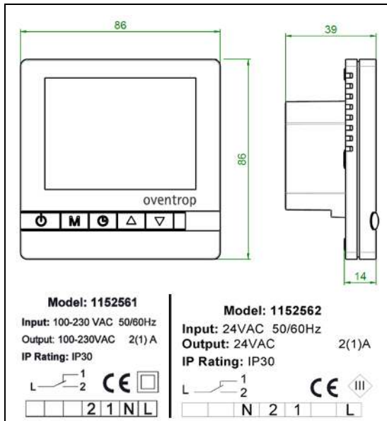
Illustr. 4.1 Dimensions
