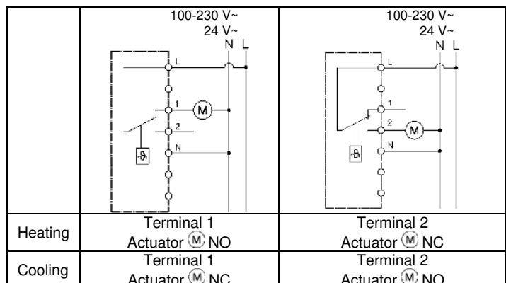
Illustr. 6.2 Wiring diagram Heating/Cooling
