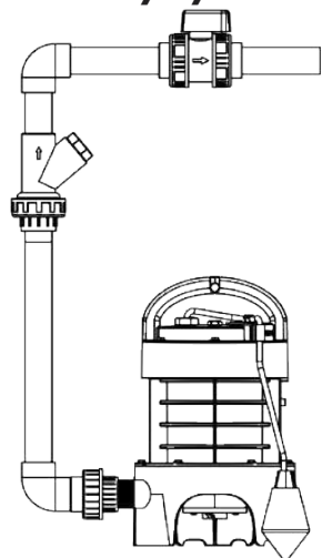
G1-1/4 pro SANIPUMP® Grinder
