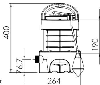
SANIPUMP® Grinder
