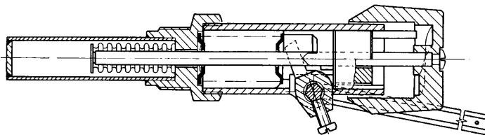
Regler "THERMOMAT RT-C"
